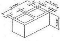
8" Double Corner
