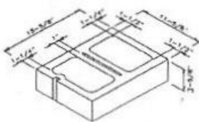
12 x 4 x 16
