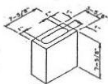
4 x 8 x 8
