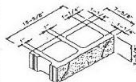
8R Half High 8 x 4 x 16 Split
