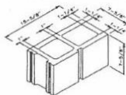
8" Single Score
