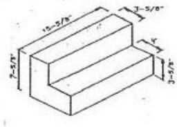
8" Solid Header
