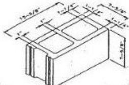
8 x 8 x 16
