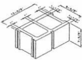
10" Single Score
