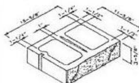
12R Half High 12 x 4 x 16 Split
