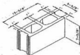
6 x 8 x 16
