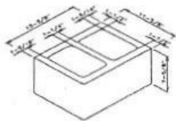
12" Single or Double Bullnose End
