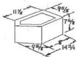
10" Quad
