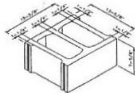
14 x 8 x 16
