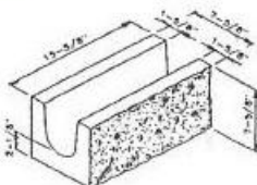
8R SBBB Solid Bottom Bond Beam
