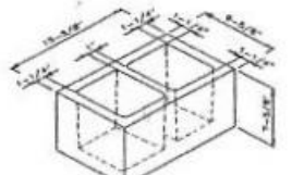
10" Solid Top
