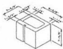
10 x 8 x 8 Sash
