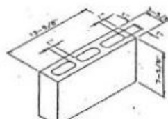
4 x 8 x 16 Hollow
