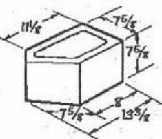
8" Quad
