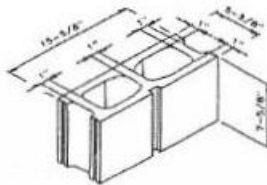
6" Single Score
