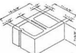
12 x 8 x 16 Sash
