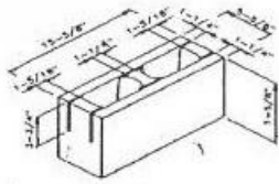
6" Hollow Bottom Bond Beam
