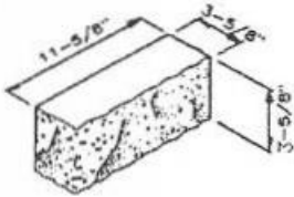
4RC Half High 4 x 4 x 12 Corner
