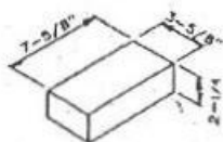
2 1/4 x 4 x 8 Cement Brick
