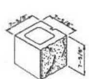
8R Half 8 x 8 x 8 Cut
