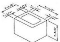
10" Half Single or
