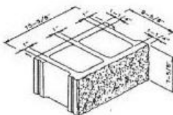
10R 10 x 8 x 16 Split
