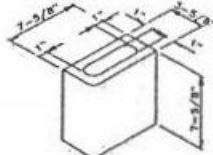
4" Half Single or Double Bullnose End
