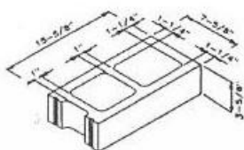
8 x 4 x 16
