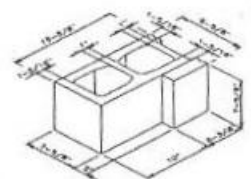
10" L Corner
