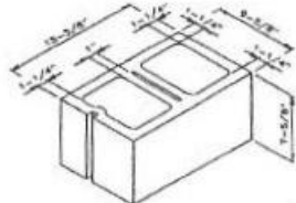
10" Sash Splittable
