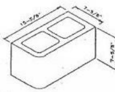
8" Single Bullnose or Double Bullnose End
