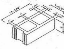
8 x 5 x 16
