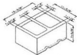
12" Weep Hole
