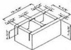
10" Hollow Bottom
