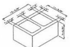
12" Double Corner
