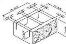
12" HBBB Hollow Bottom Bond Beam
