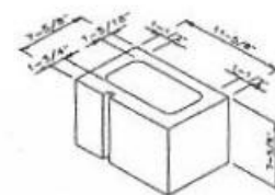
12 x 8 x 8 Sash
