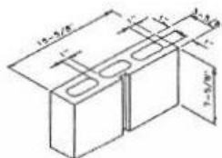
4" Single Score
