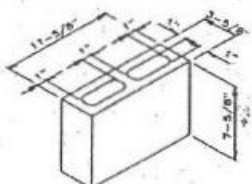
4 x 8 x 12 Hollow Starter
