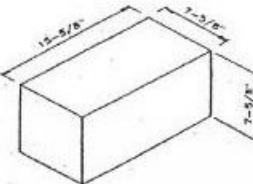
8" Solid
