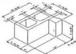
12" L Corner
