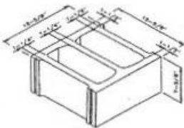
16 x 8 x 16
