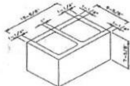
10" Double Corner
