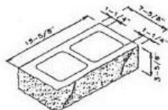
8RC Half High 8 x 4 x 16 Corner
