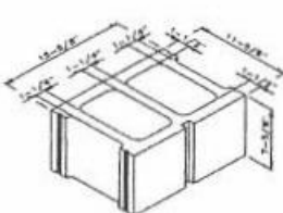
12" Single Score
