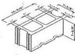
8" Weep Hole
