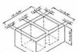
12" Solid Top
