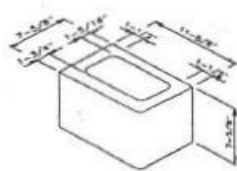
12" Half Single or Double Bullnose
