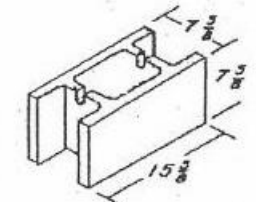
8" Ivory
