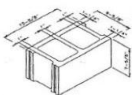
10" Stretcher
