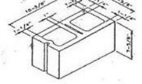
8" Whole Sash Splittable
