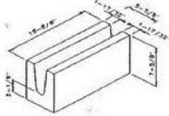
6" Solid Bottom Bond Beam
