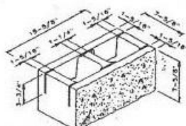
8R HBBB Hollow Bottom Bond Beam
