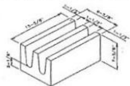
10" Solid Bottom
